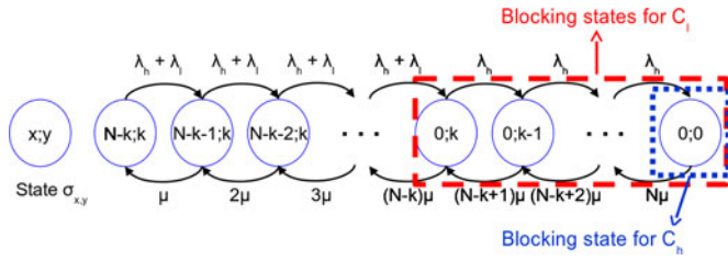
Fig. 2. Markov chain for the single node model without wake-up time.
