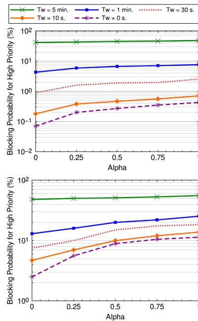
Fig. 10. Blocking as a function of \alpha for the opaque (top) and translucent (bottom) cases for the CORONET network scenario.
