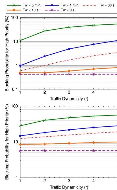
Fig. 7. Blocking as a function of r for the opaque (top) and translucent (bottom) cases for the CORONET network scenario without WTAR.
