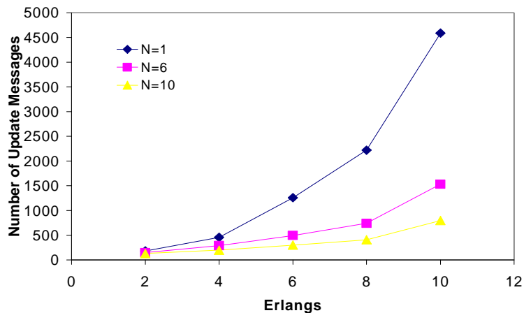
Figure 3. Number of update messages
