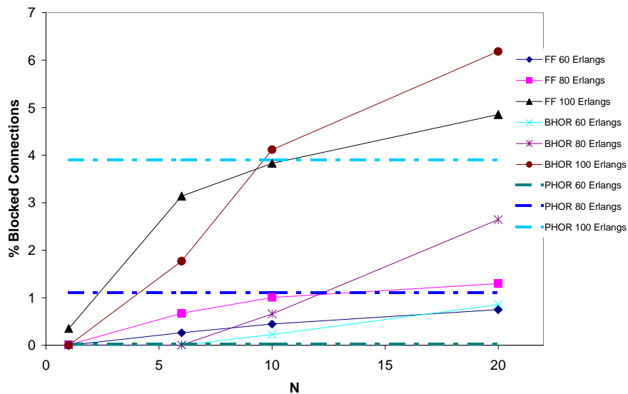
Figure 6. Connection blocking for the First-Fit, the BHOR and the PHOR algorithms depending on the updating frequency
