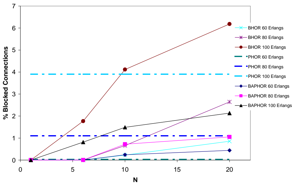
Figure 8. Connection blocking for the BHOR and the PHOR algorithms depending on the updating frequency
