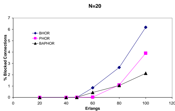
7.d. Results for N=20.
